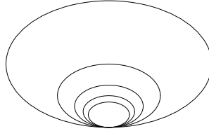
Figure 1: The Hawaiian earring
